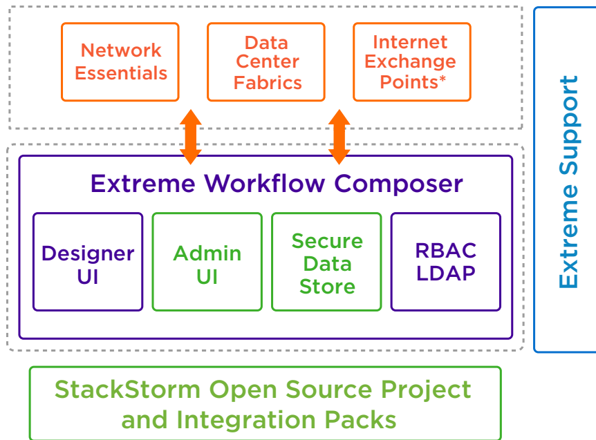
Figure 5: The Extreme Workflow Composer Automation Suite Architecture.
